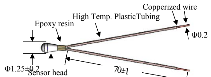
Figure 2. Side View of ATH100K1R25T70S
