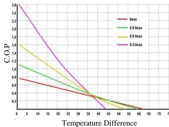
Figure 5. C.O.P vs. Temperature Difference
