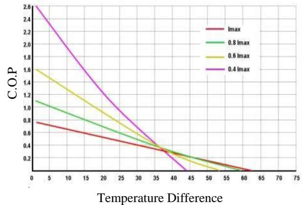
Figure 5. C.O.P vs. Temperature Difference
