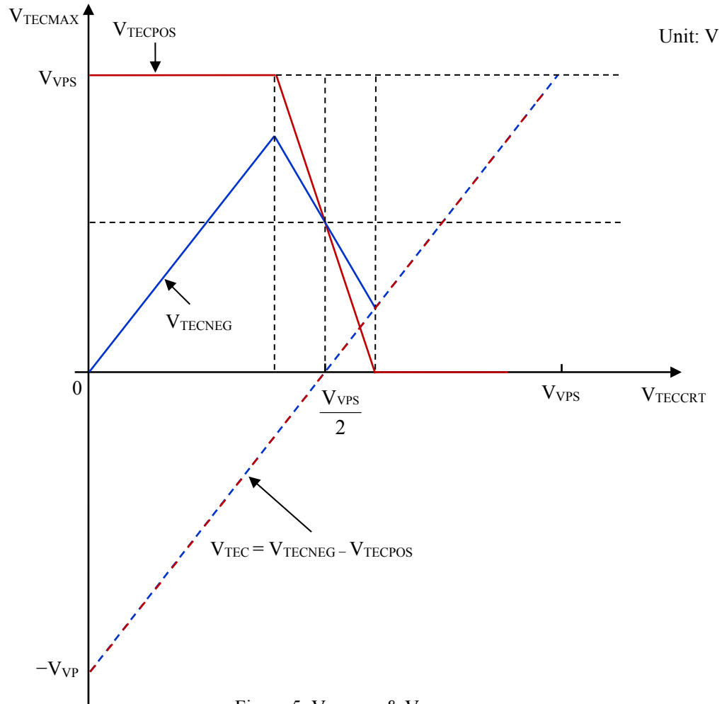
Figure 5. V_{TEC\text{MAX}} & V_{TEC\text{CRT}}
