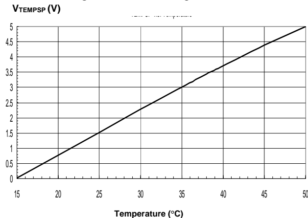
Figure 8. TEMPSP vs. Temperature
