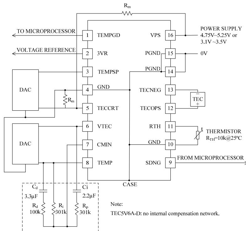
Figure 4. TEC Controller Connections
