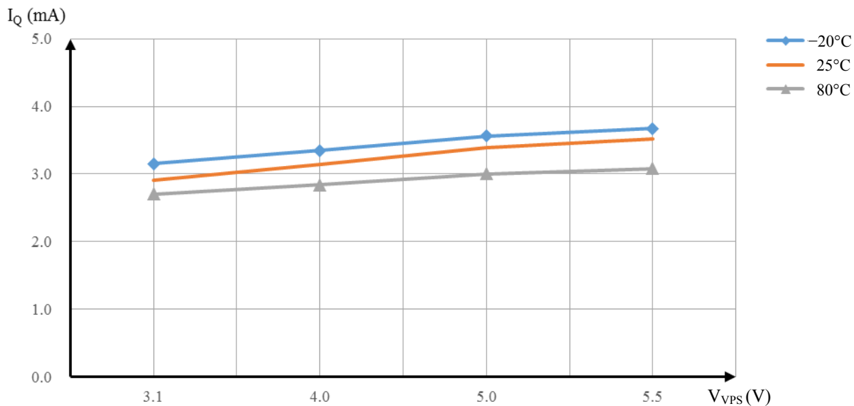
Figure 14. VPS and Temperature vs. I_Q
