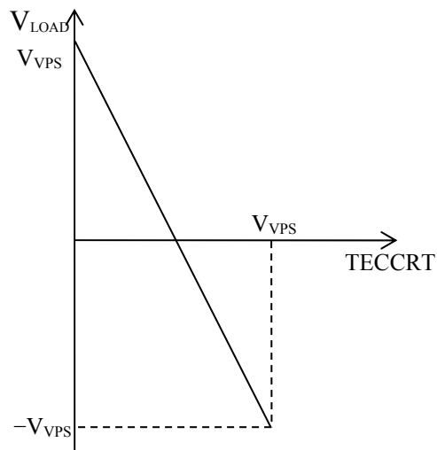
Figure 13. V_{LOAD} vs. TECVRT
